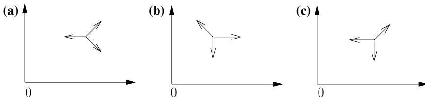
Fig. 4.1 Three examples of groups of order 6
